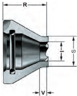
A14 Driving discs, with interchangeable carbide driving plates 9.5 x 3.2, right- and left-hand rotation, max. workpiece hardness 40 HRC
