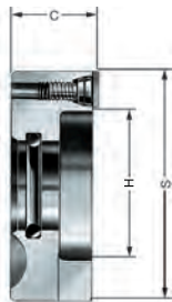
A14 Driving discs, with interchangeable carbide driving plates 9.5 x 3.2, right- and left-hand rotation, max. workpiece hardness 40 HRC
