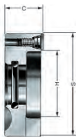
A14 Driving discs, with interchangeable carbide driving plates 9.5 x 3.2, right-hand rotation, max. workpiece hardness 40 HRC
