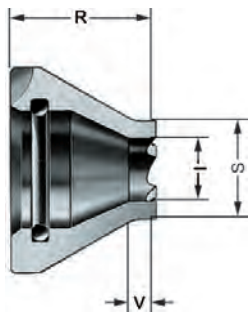
A14 Driving discs, toothed, left-hand rotation, max. workpiece hardness 35 HRC
