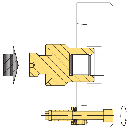
Quick-acting bolt backed off 1/2 turn
