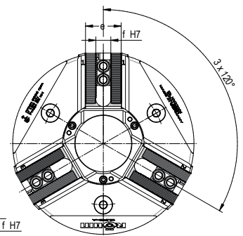
offsetted T-nut only in size 254
