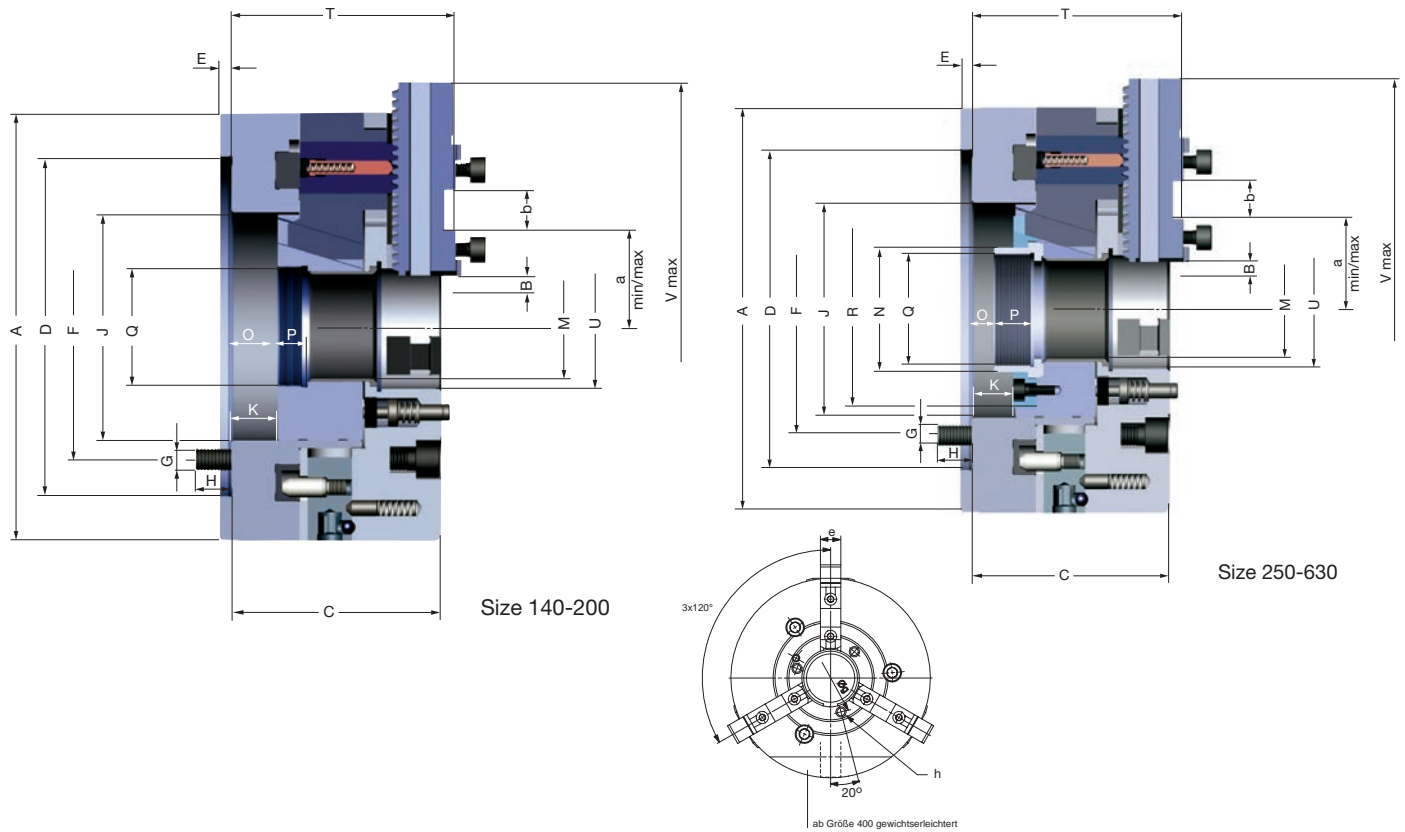
C 15 3-jaws power chuck DURO-NC, with quick jaw change systems, central jaw unlocking, angle-serrated Cylindrical centre mount, mounting dimensions to DIN 6353
