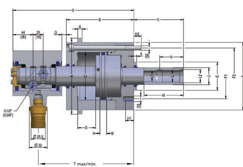
C 15 Oil-operated actuating cylinders without through-hole OVS, basic model, with safety device, up to 80 bar - Steel design for high speed, fastening from the rear, central through-hole
