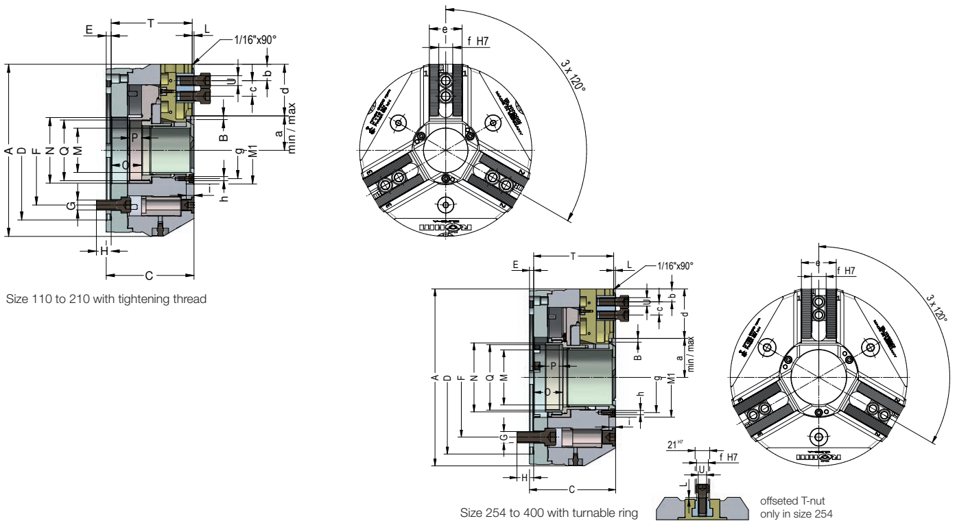
Size 254 to 400 with turnable ring
